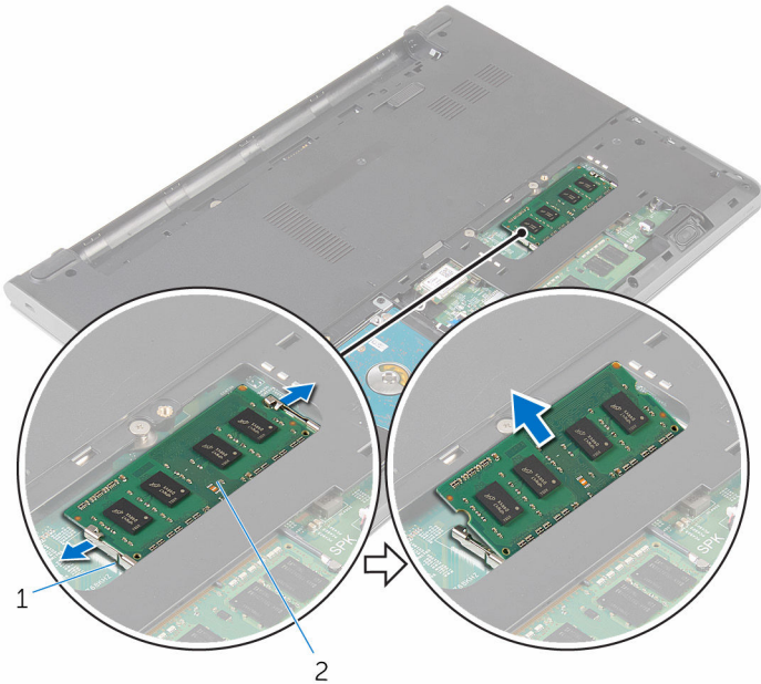
1 securing clips (2)
